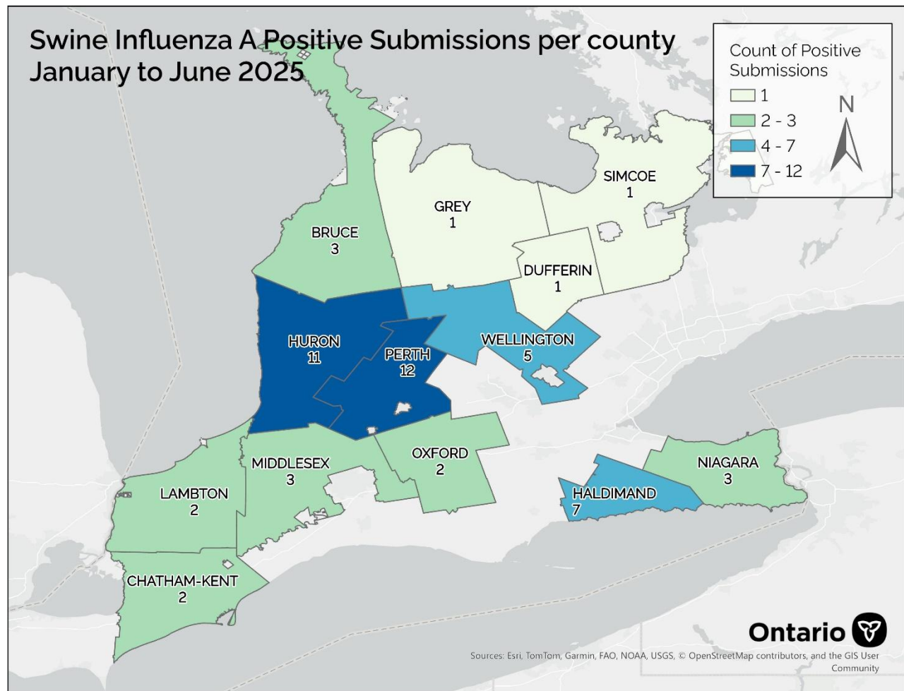
Figure 7. Submissions positive for influenza (not including ELISA tests) in swine by county, Ontario, January 2025 to June 2025.
